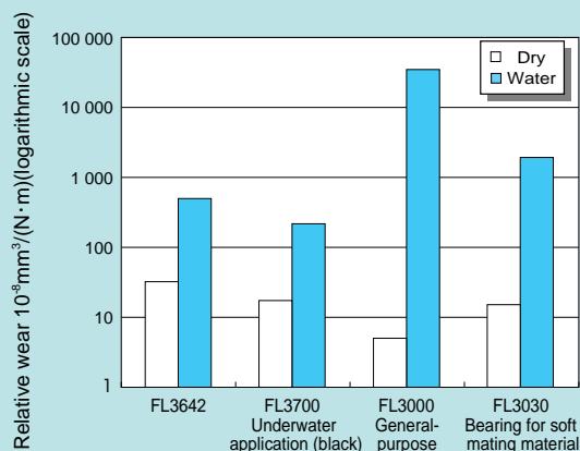
Comparison of relative wear of FL3642 with other NTN bearing materials
