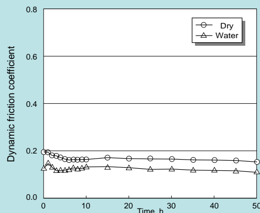
Time-dependent change in dynamic friction coefficient, either in a dry state or with water lubrication.
